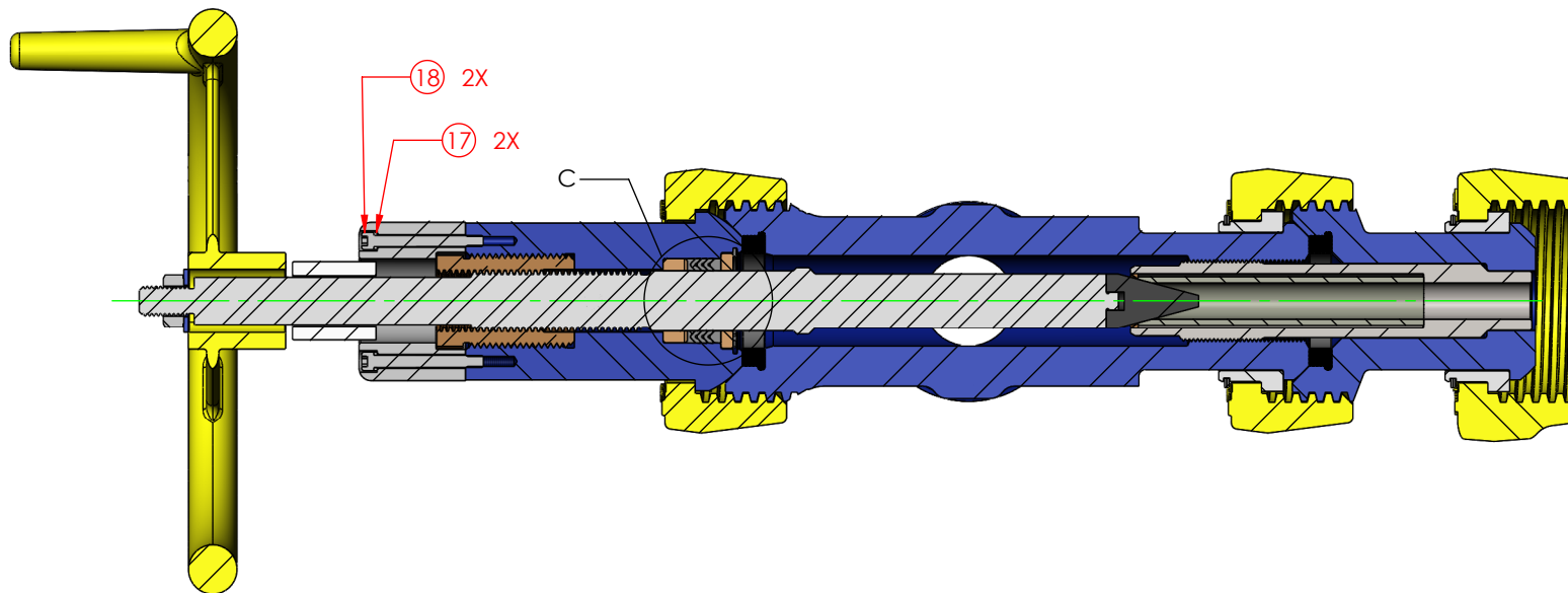
SECTION B-B
