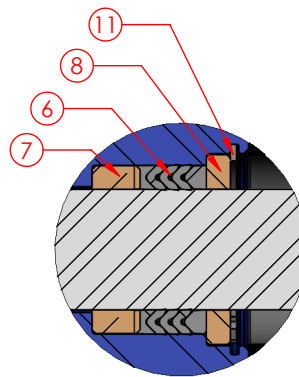
DETAIL C B5 PACKING ORIENTATION
