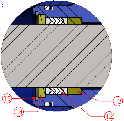
DETAIL A PACKING ORIENTATION
