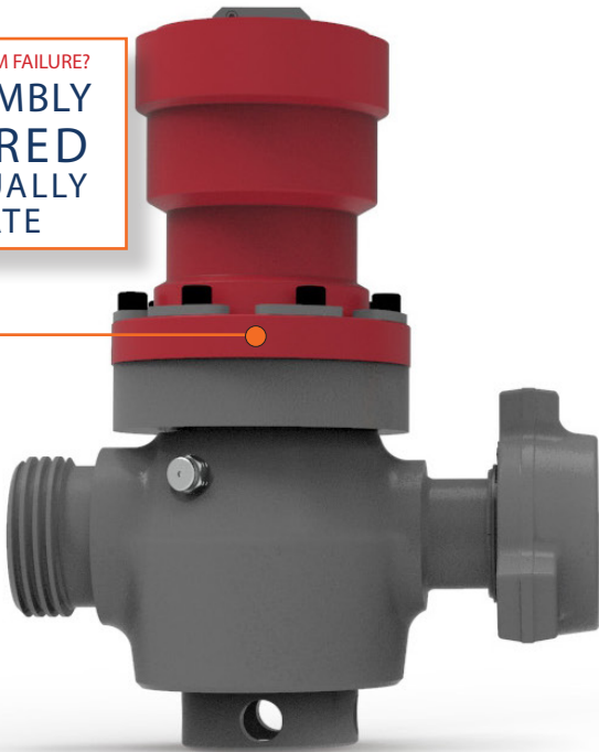
VALVE-LT, 2X2"1502 (HYD ACTUATED w/BRAND-X) TOTAL WEIGHT: 165 LBS
